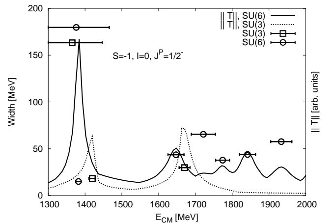
Fig. 1. Spin-parity J^P = \frac{1}{2}^- resonance properties in the I=0, S=-1 ( Y=0 ) sector. Solid and dotted lines stand for the SU(6) and SU(3) T -matrix norms, respectively. The norm is calculated as \|T\| = \text{Max}(\sum_{j=1}^n |T_{ij}|, i=1, \dots, n) where i, j run over the number of coupled channels. Finally, the points with error bars are defined from the masses and widths of the found resonances as (M_R \pm \Gamma_R/2, \Gamma_R) .
